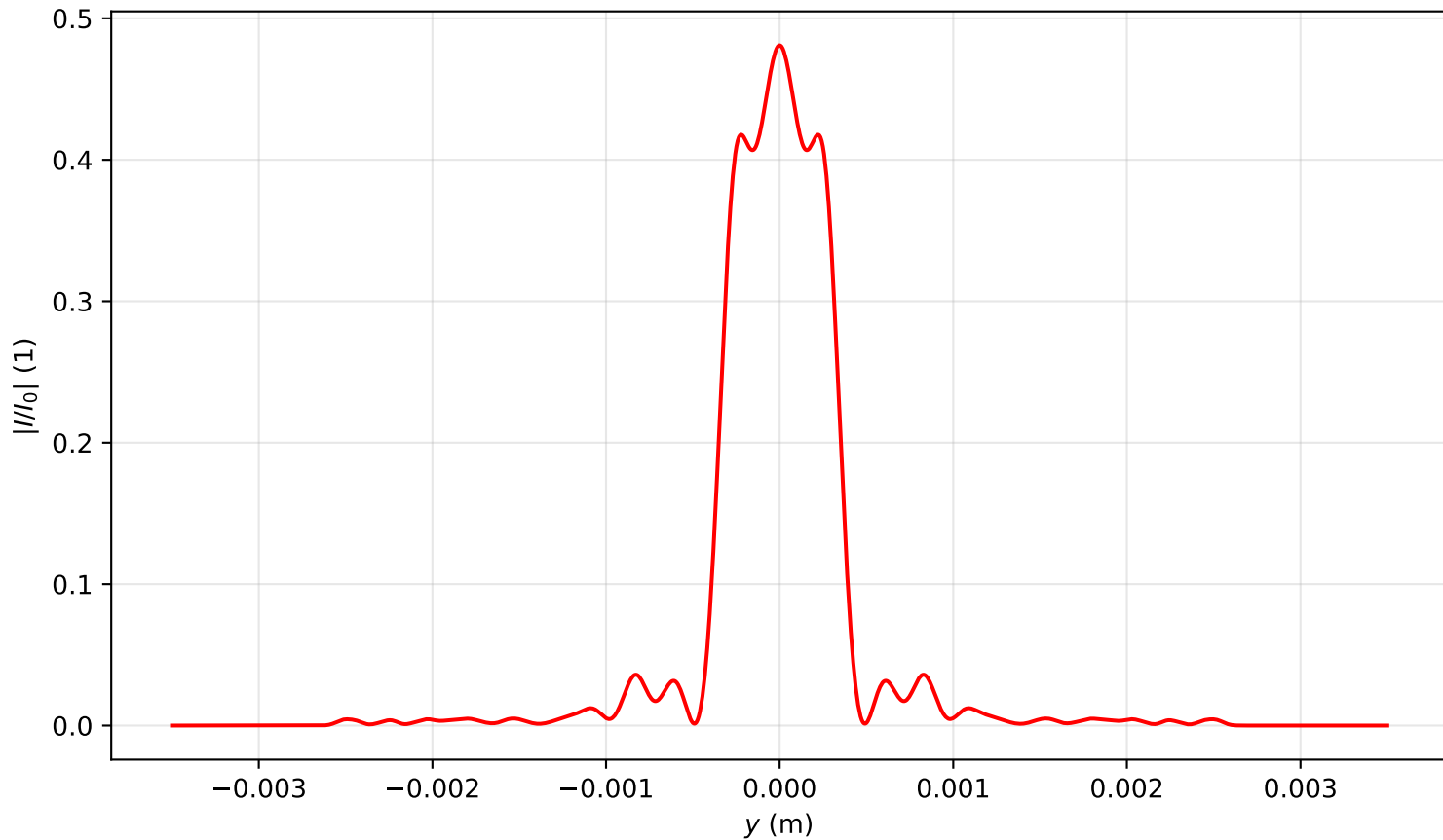
Intensity profile I(x=0, y, z=1.911)/I_0 , P_{in}=13.0\text{Pcr} , artificial time
