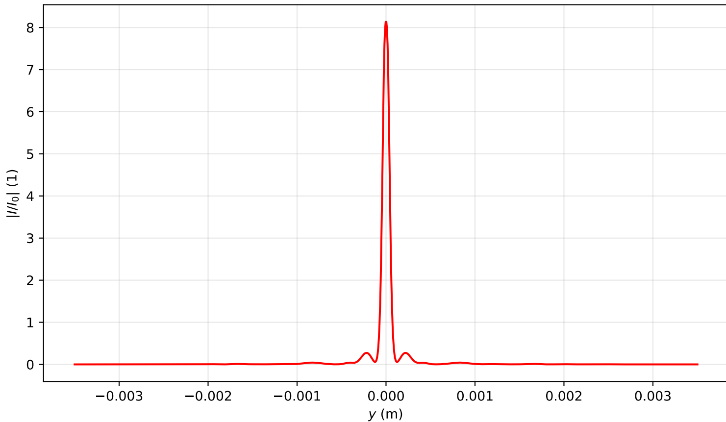
Intensity profile I(x=0, y, z=2.149)/I_0 , P_{in}=13.0P_{cr} , artificial time
