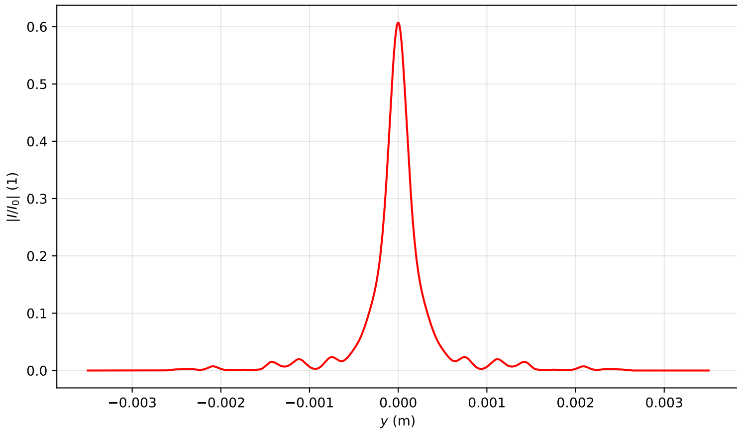
Intensity profile I(x=0, y, z=2.627)/I_0 , P_{in}=13.0P_{cr} , artificial time
