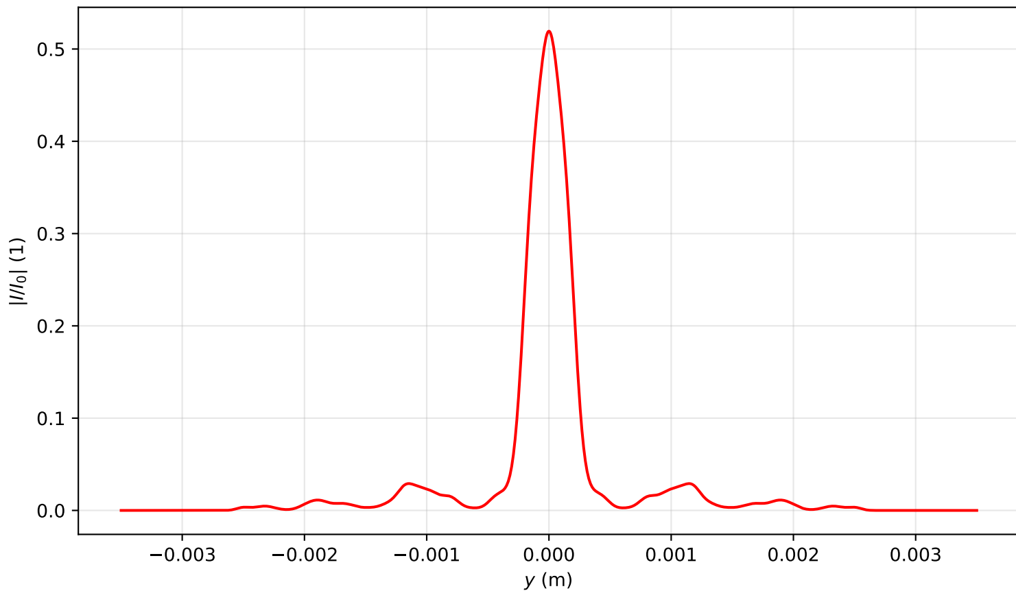
Intensity profile I(x=0, y, z=3.105)/I_0 , P_{in}=13.0P_{cr} , artificial time
