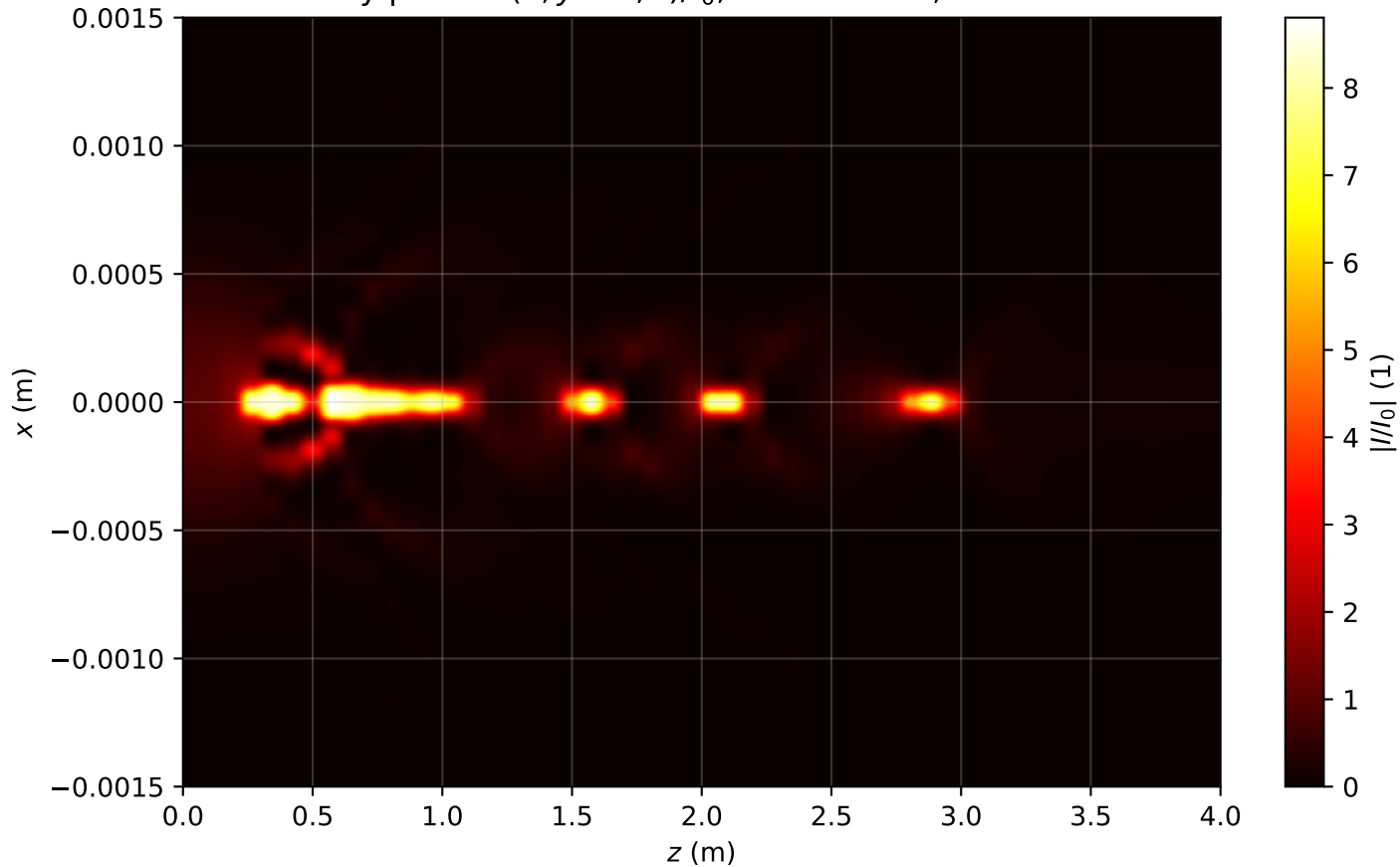
Intensity profile I(x, y = 0, z)/I_0 , P_{in}=13.0P_{cr} , artificial time
