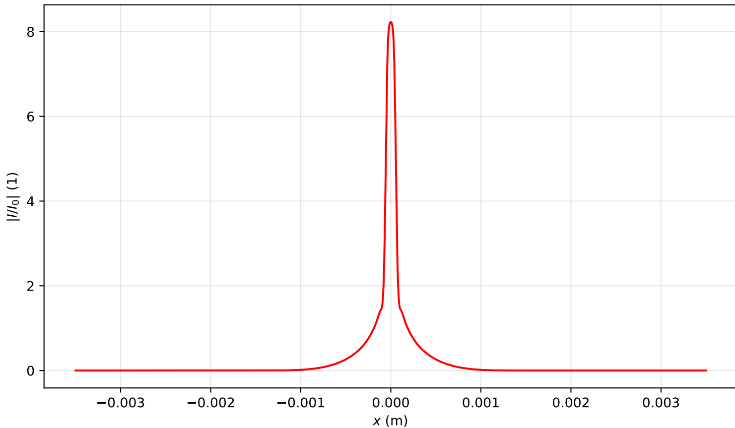
Intensity profile I(x, y = 0, z = 0.239)/I_0 , P_{in}=13.5P_{cr} , artificial time
