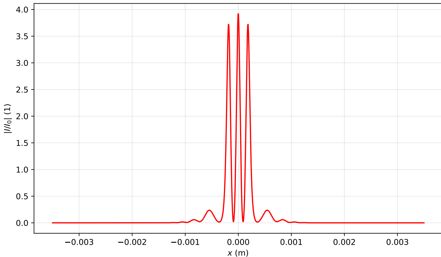
Intensity profile I(x, y = 0, z = 0.478)/I_0 , P_{in}=13.5P_{cr} , artificial time
