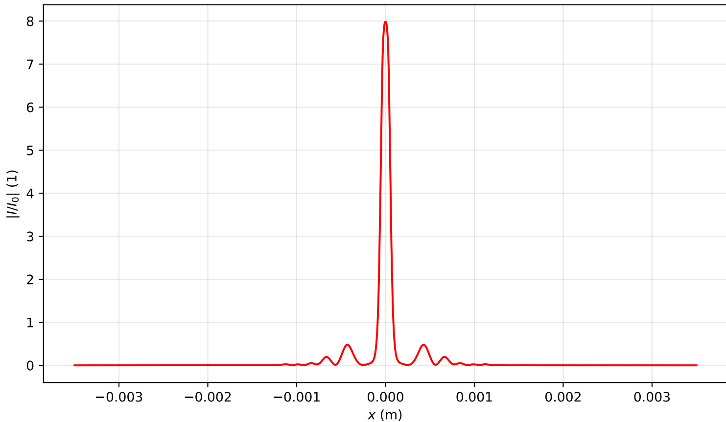
Intensity profile I(x, y = 0, z = 0.716)/I_0 , P_{in}=13.5P_{cr} , artificial time
