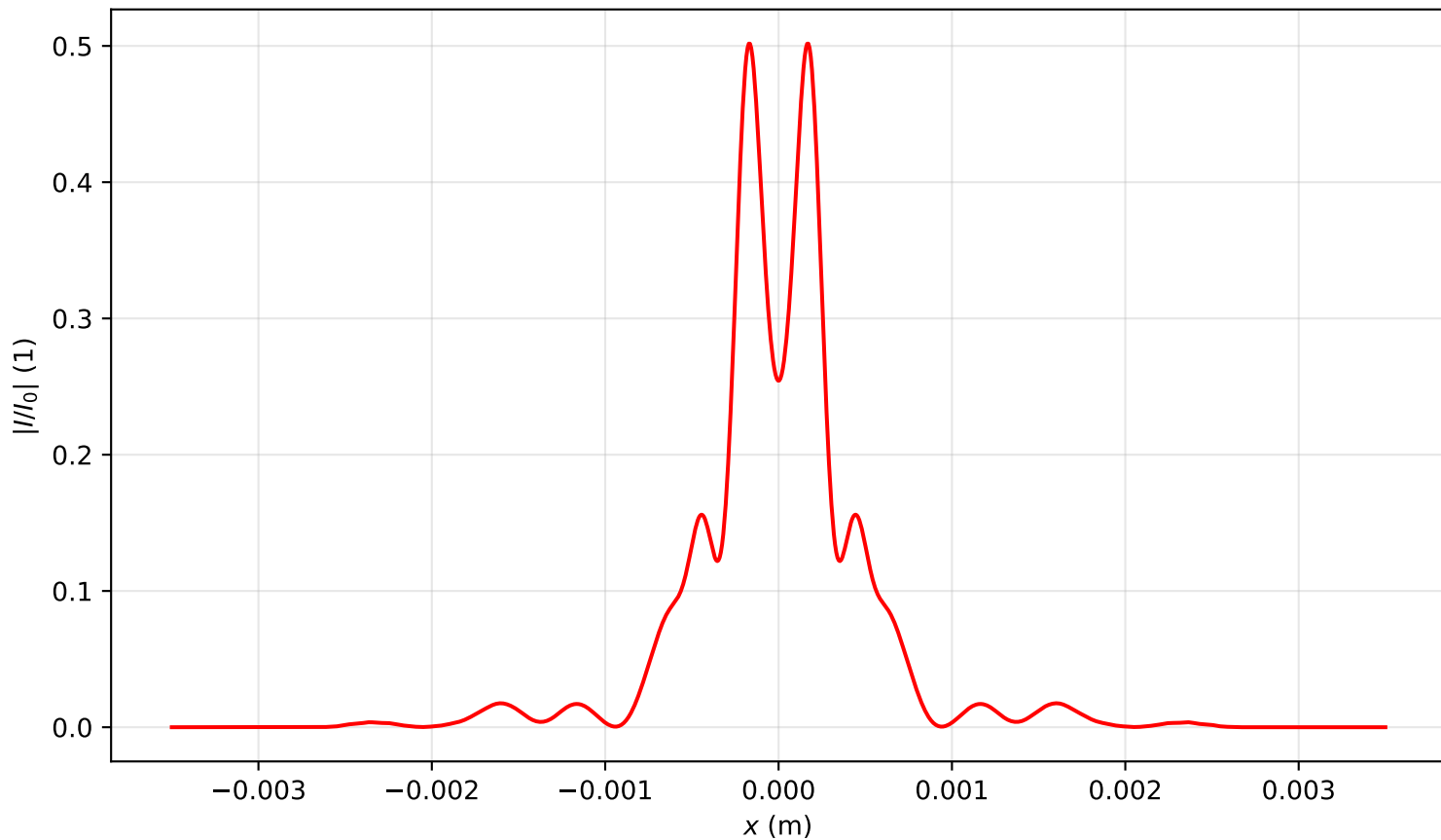
Intensity profile I(x, y = 0, z = 1.194)/I_0 , P_{in}=13.5P_{cr} , artificial time
