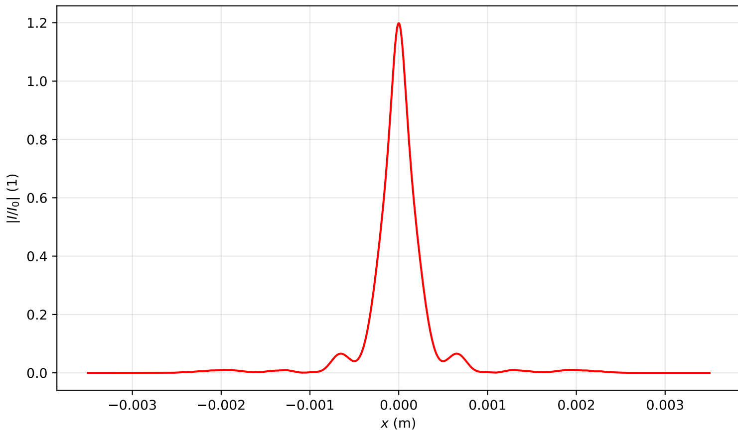
Intensity profile I(x, y = 0, z = 1.433)/I_0 , P_{in}=13.5P_{cr} , artificial time
