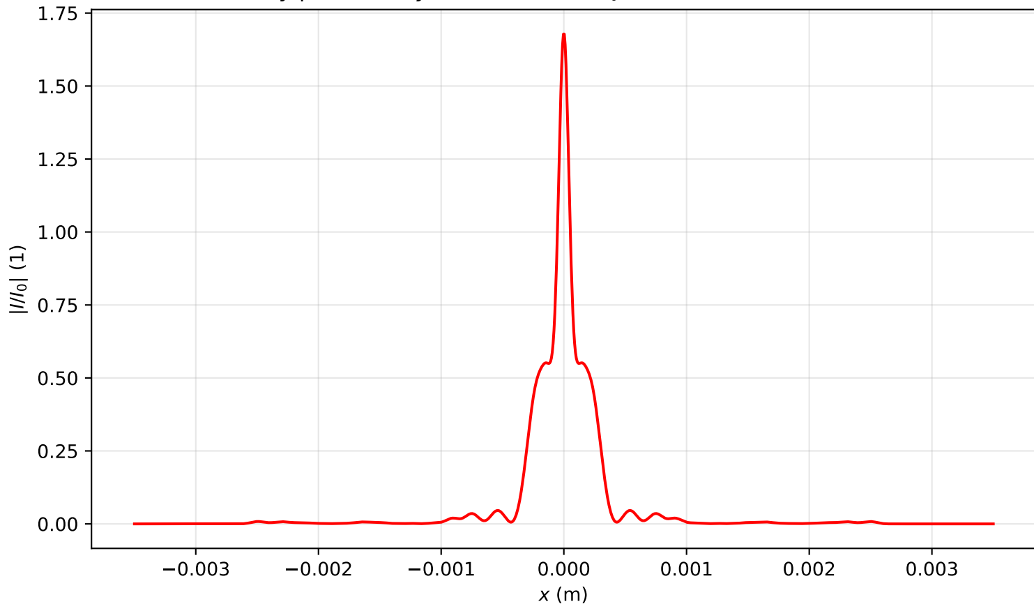
Intensity profile I(x, y = 0, z = 1.672)/I_0 , P_{in}=13.5P_{cr} , artificial time
