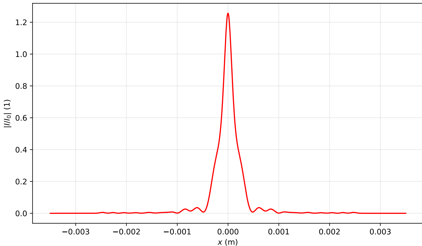
Intensity profile I(x, y = 0, z = 1.911)/I_0 , P_{in}=13.5P_{cr} , artificial time
