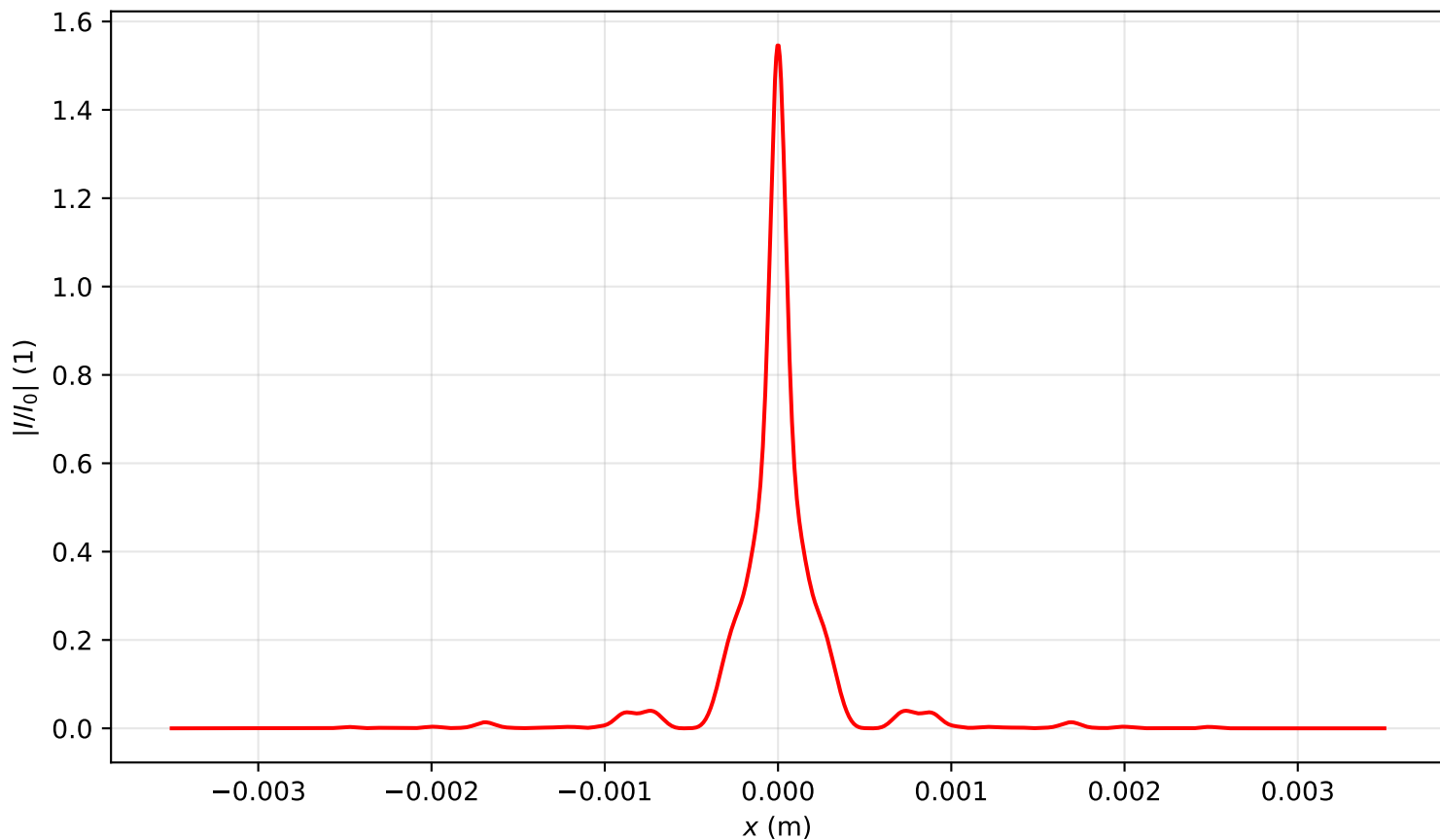
Intensity profile I(x, y = 0, z = 2.149)/I_0 , P_{in}=13.5P_{cr} , artificial time
