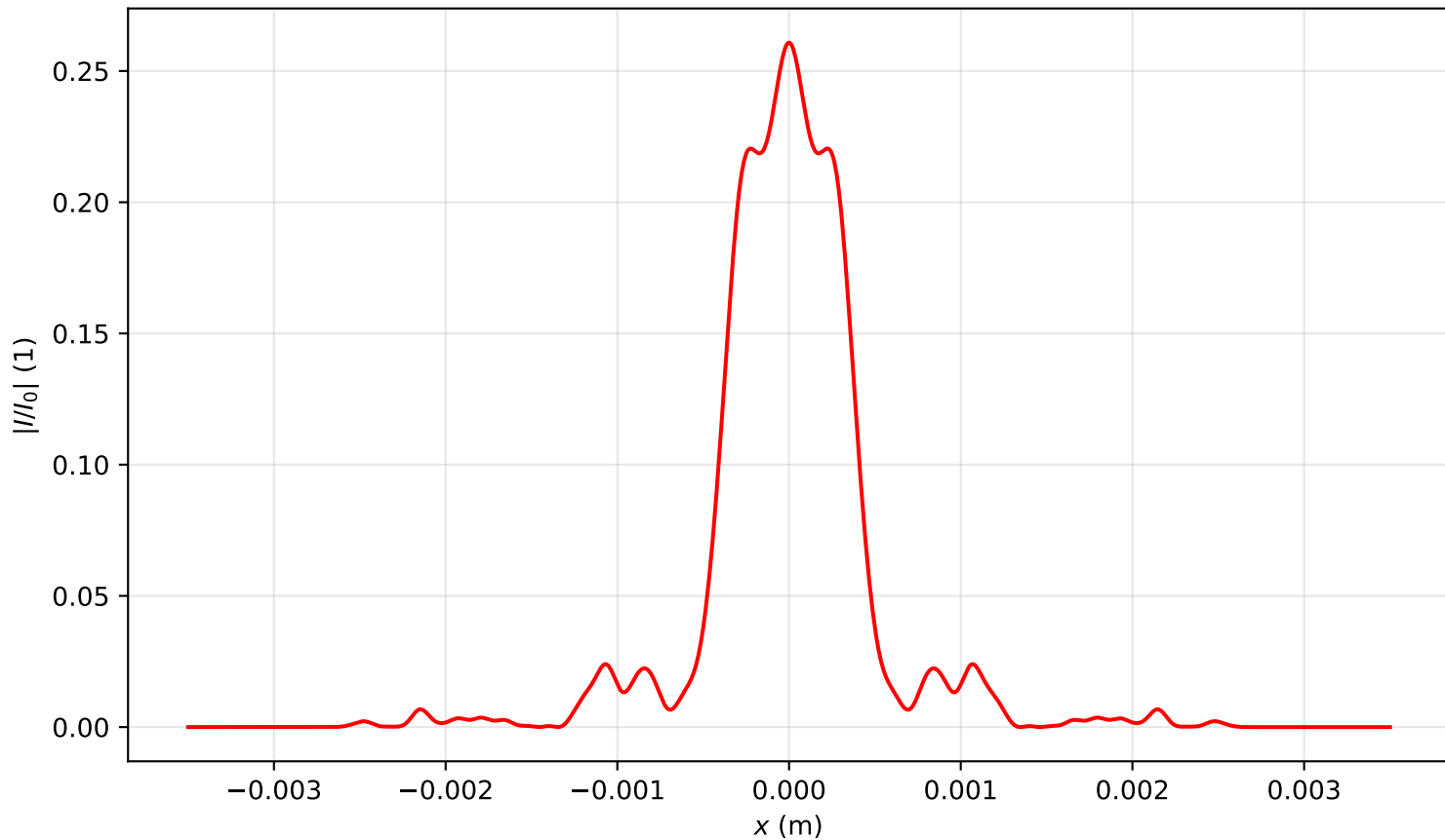
Intensity profile I(x, y = 0, z = 2.388)/I_0 , P_{in}=13.5P_{cr} , artificial time
