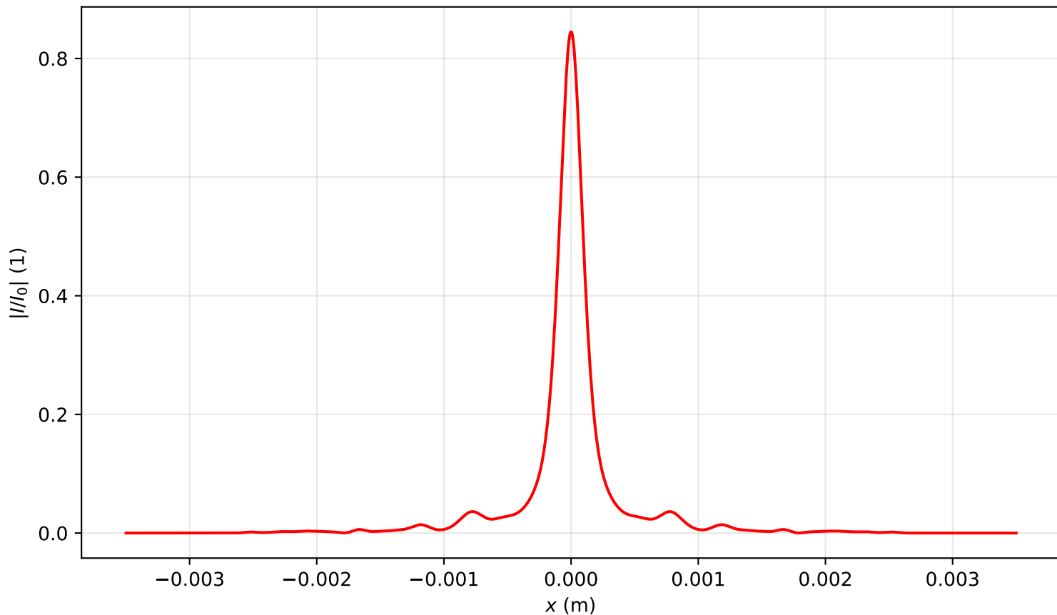
Intensity profile I(x, y = 0, z = 2.627)/I_0 , P_{in}=13.5P_{cr} , artificial time
