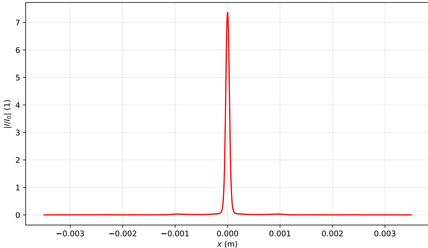
Intensity profile I(x, y = 0, z = 2.866)/I_0 , P_{in}=13.5P_{cr} , artificial time
