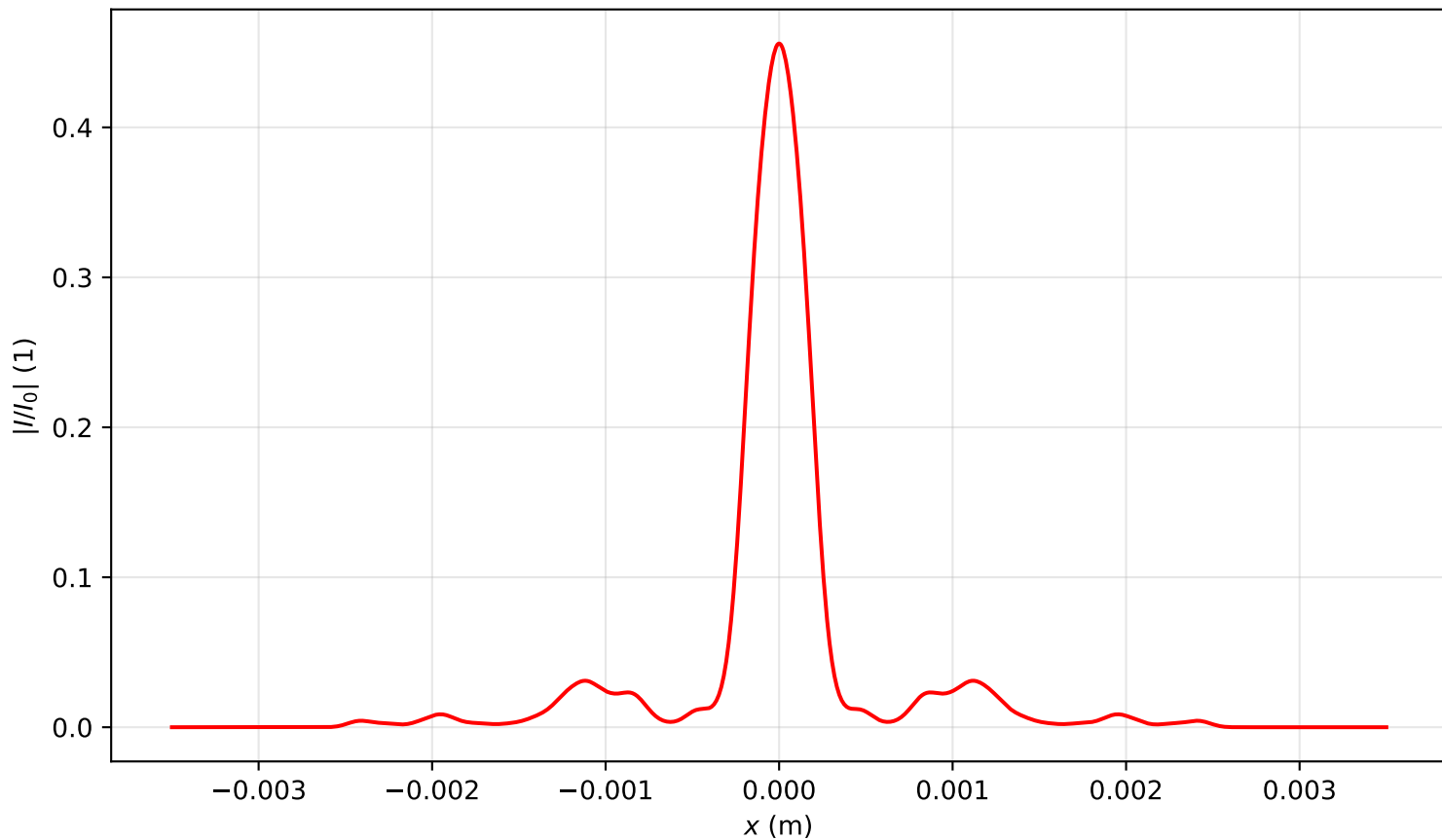
Intensity profile I(x, y = 0, z = 3.105)/I_0 , P_{in}=13.5P_{cr} , artificial time
