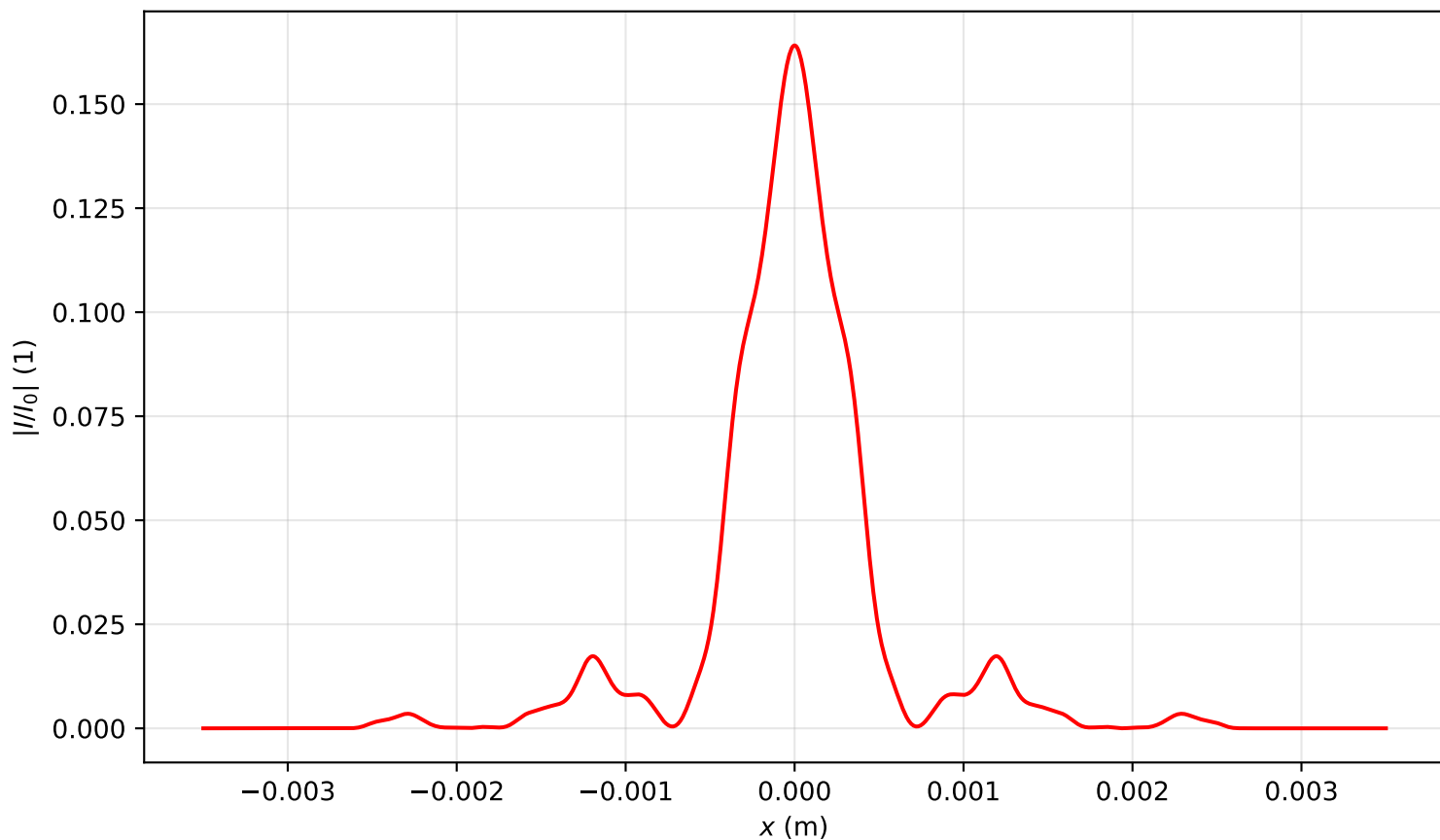
Intensity profile I(x, y = 0, z = 3.344)/I_0 , P_{in}=13.5P_{cr} , artificial time
