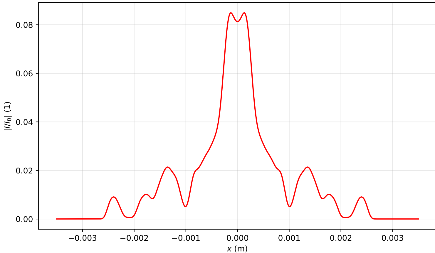
Intensity profile I(x, y = 0, z = 3.582)/I_0 , P_{in}=13.5P_{cr} , artificial time
