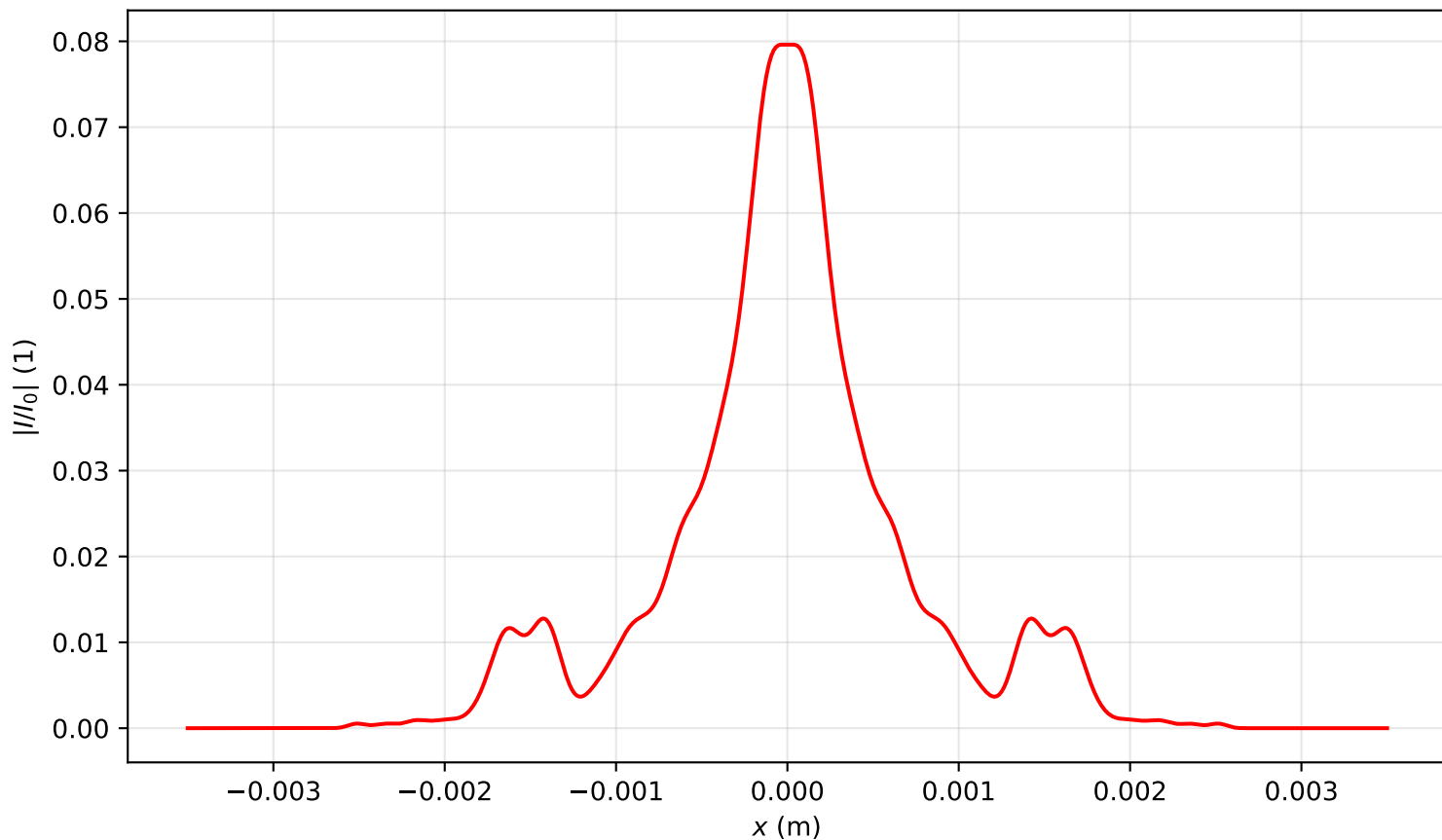
Intensity profile I(x, y = 0, z = 3.821)/I_0 , P_{in}=13.5P_{cr} , artificial time
