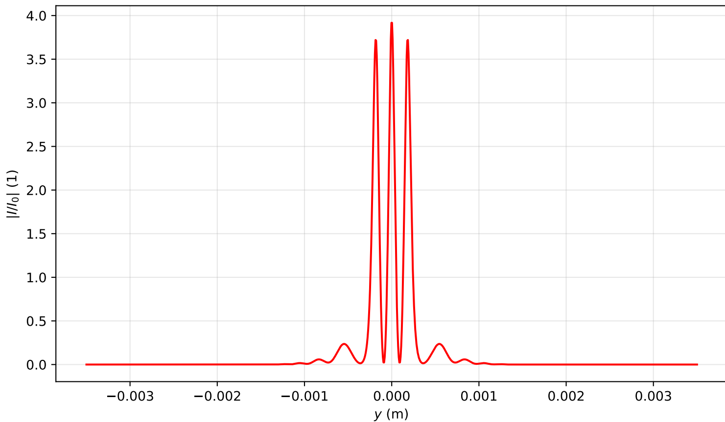
Intensity profile I(x=0, y, z=0.478)/I_0 , P_{in}=13.5P_{cr} , artificial time
