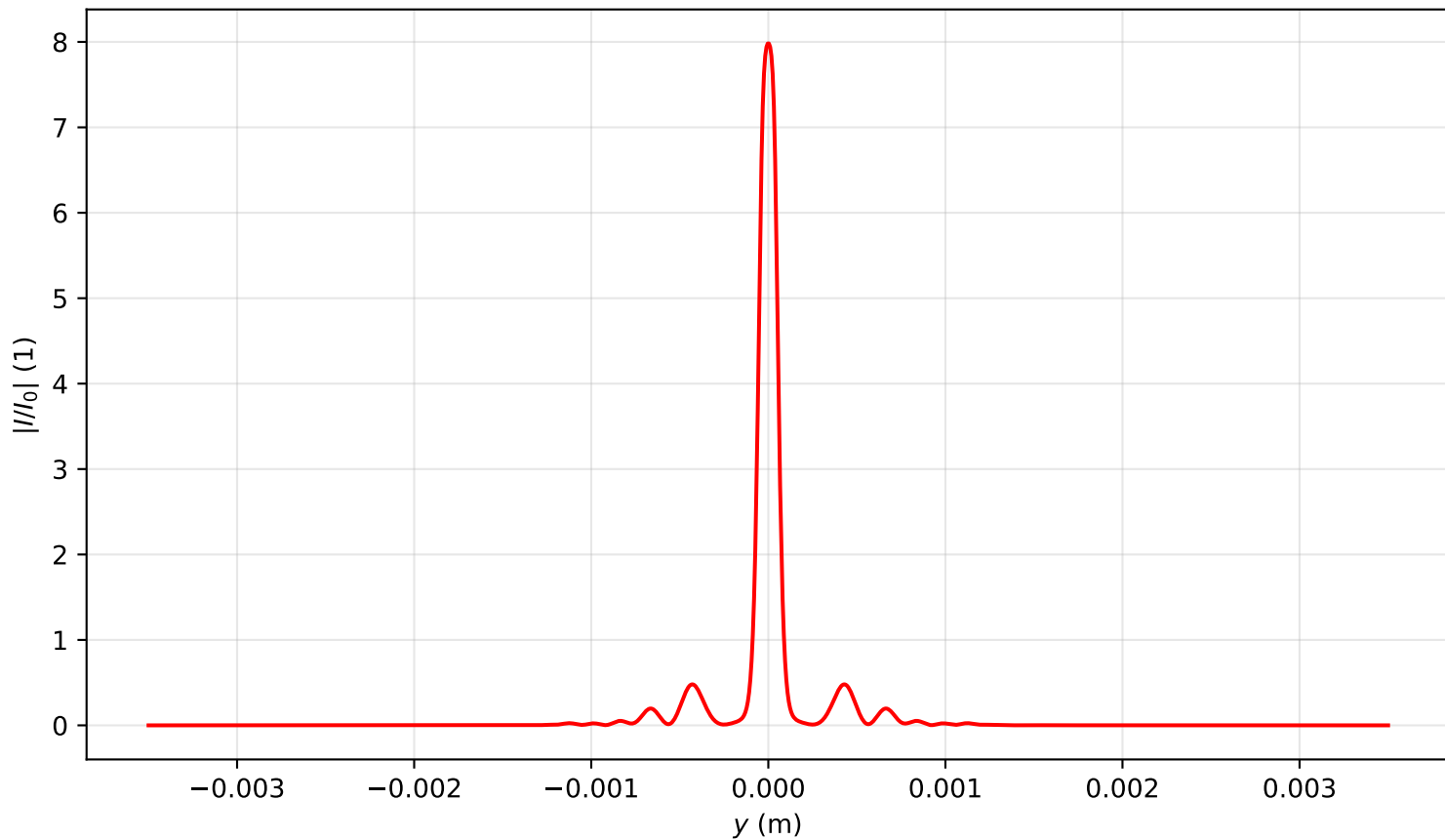
Intensity profile I(x=0, y, z=0.716)/I_0 , P_{in}=13.5P_{cr} , artificial time
