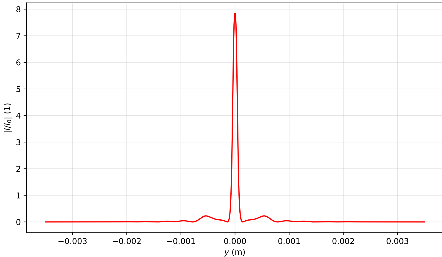
Intensity profile I(x=0, y, z=0.955)/I_0 , P_{in}=13.5P_{cr} , artificial time
