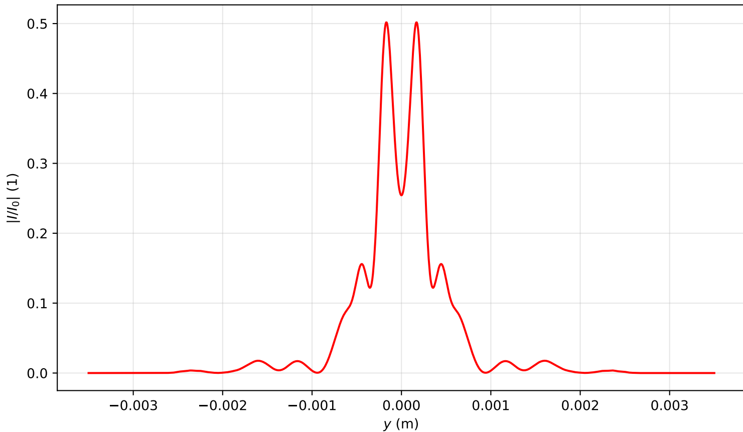
Intensity profile I(x=0, y, z=1.194)/I_0 , P_{in}=13.5P_{cr} , artificial time
