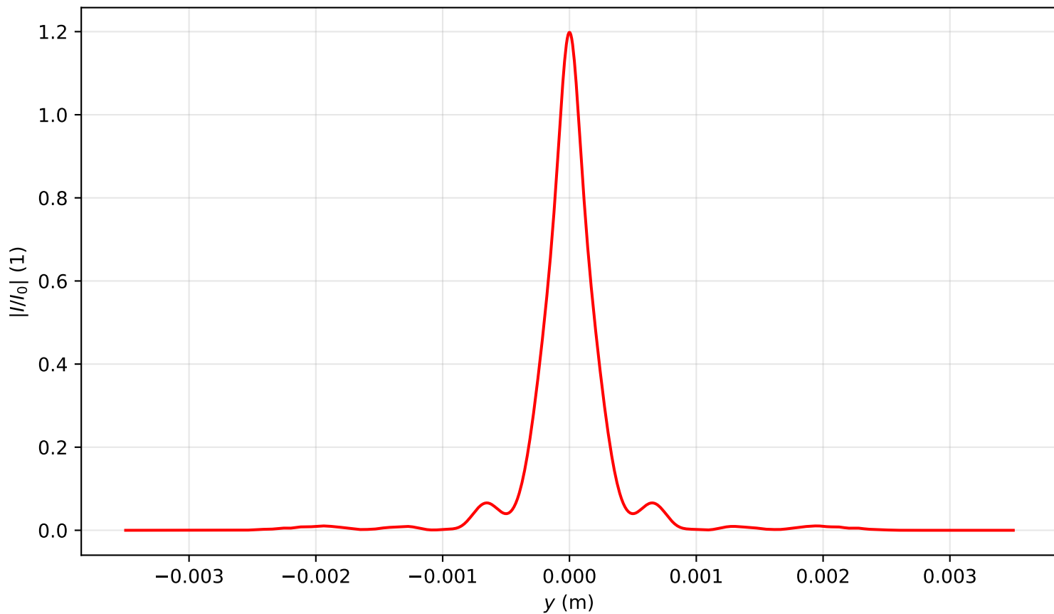
Intensity profile I(x=0, y, z=1.433)/I_0 , P_{in}=13.5P_{cr} , artificial time
