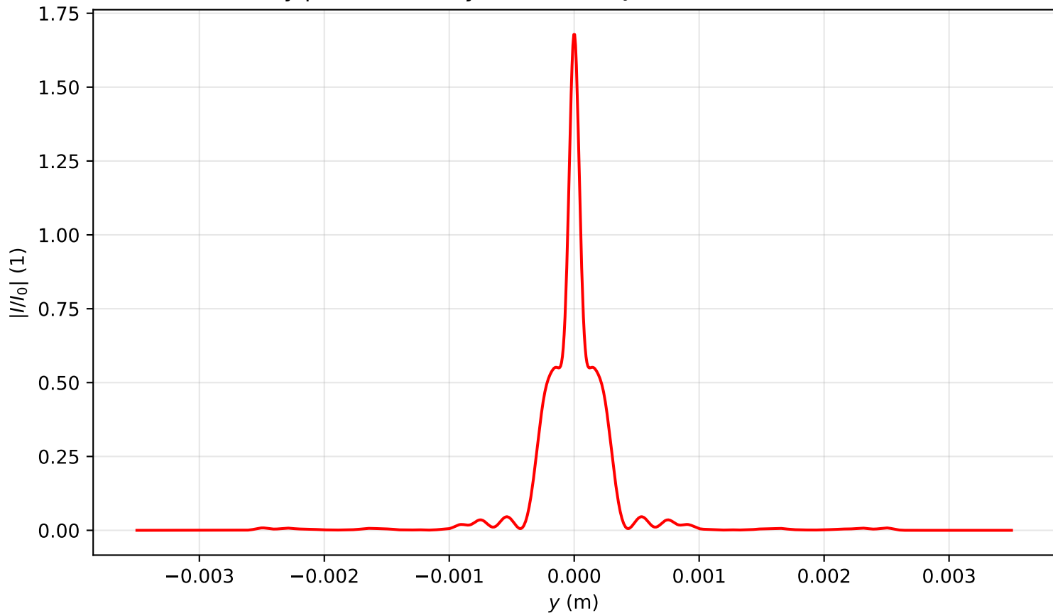
Intensity profile I(x=0, y, z=1.672)/I_0 , P_{in}=13.5P_{cr} , artificial time
