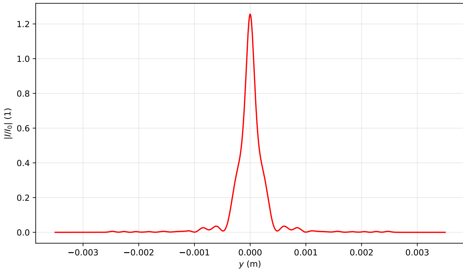
Intensity profile I(x=0, y, z=1.911)/I_0 , P_{in}=13.5P_{cr} , artificial time
