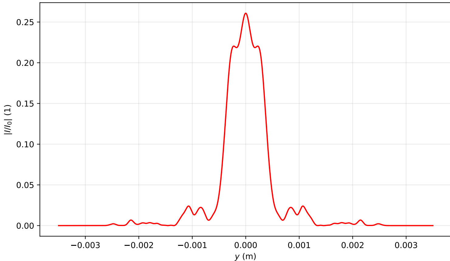
Intensity profile I(x=0, y, z=2.388)/I_0 , P_{in}=13.5P_{cr} , artificial time
