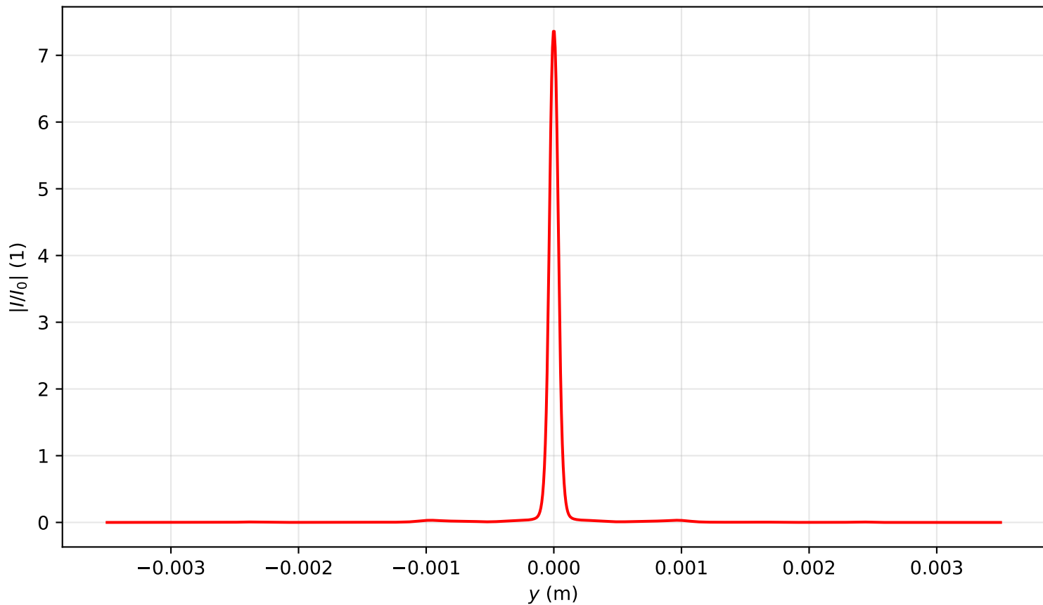
Intensity profile I(x=0, y, z=2.866)/I_0 , P_{in}=13.5P_{cr} , artificial time
