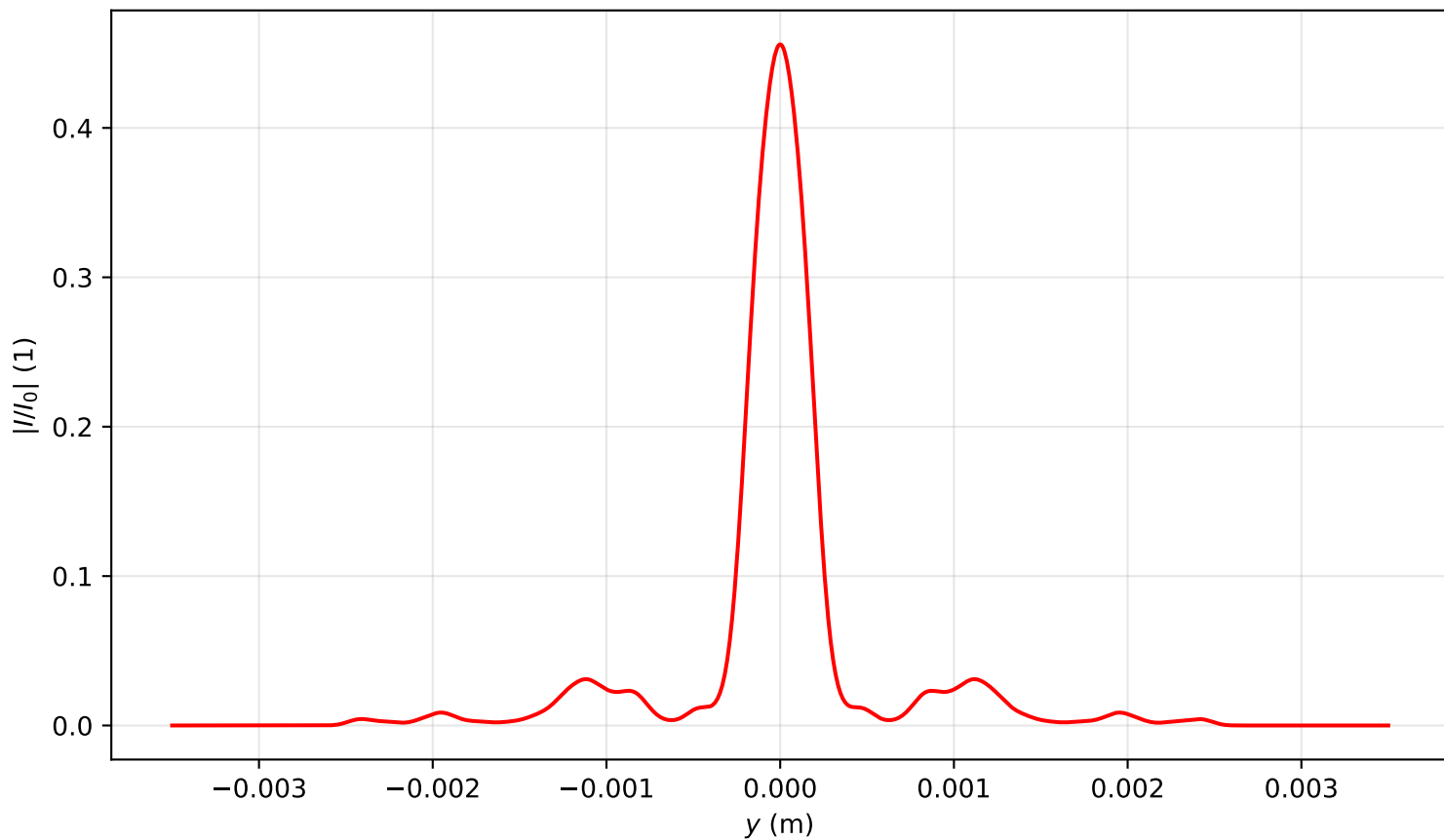
Intensity profile I(x=0, y, z=3.105)/I_0 , P_{in}=13.5P_{cr} , artificial time
