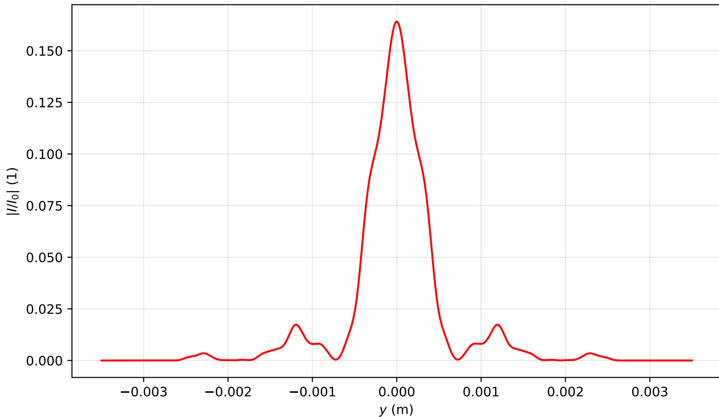
Intensity profile I(x = 0, y, z = 3.344)/I_0 , P_{in}=13.5P_{cr} , artificial time
