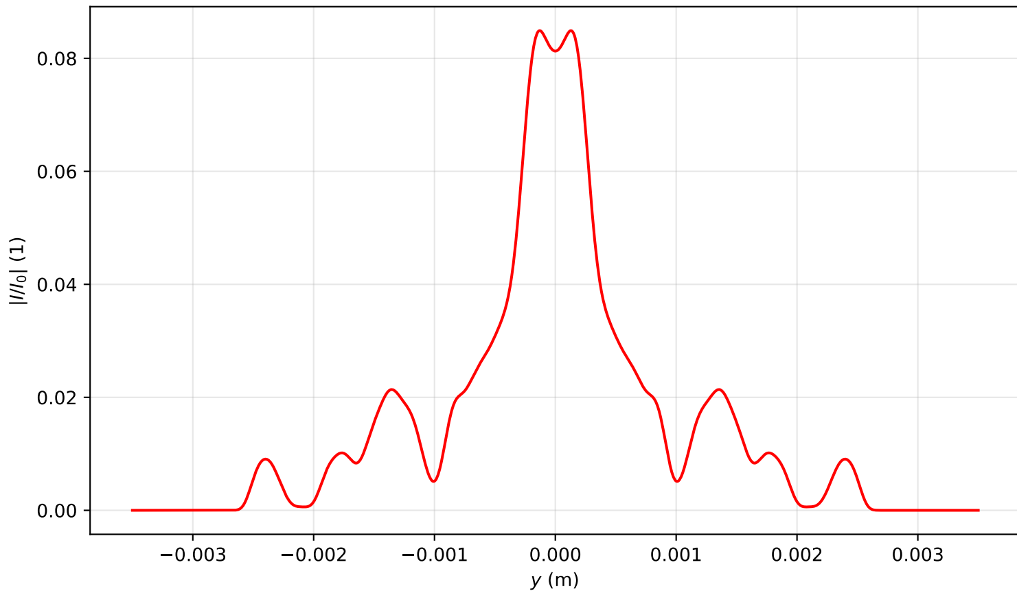
Intensity profile I(x = 0, y, z = 3.582)/I_0 , P_{in}=13.5P_{cr} , artificial time
