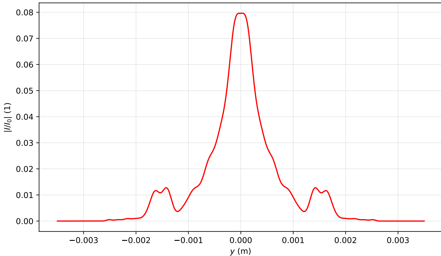
Intensity profile I(x = 0, y, z = 3.821)/I_0 , P_{in}=13.5P_{cr} , artificial time
