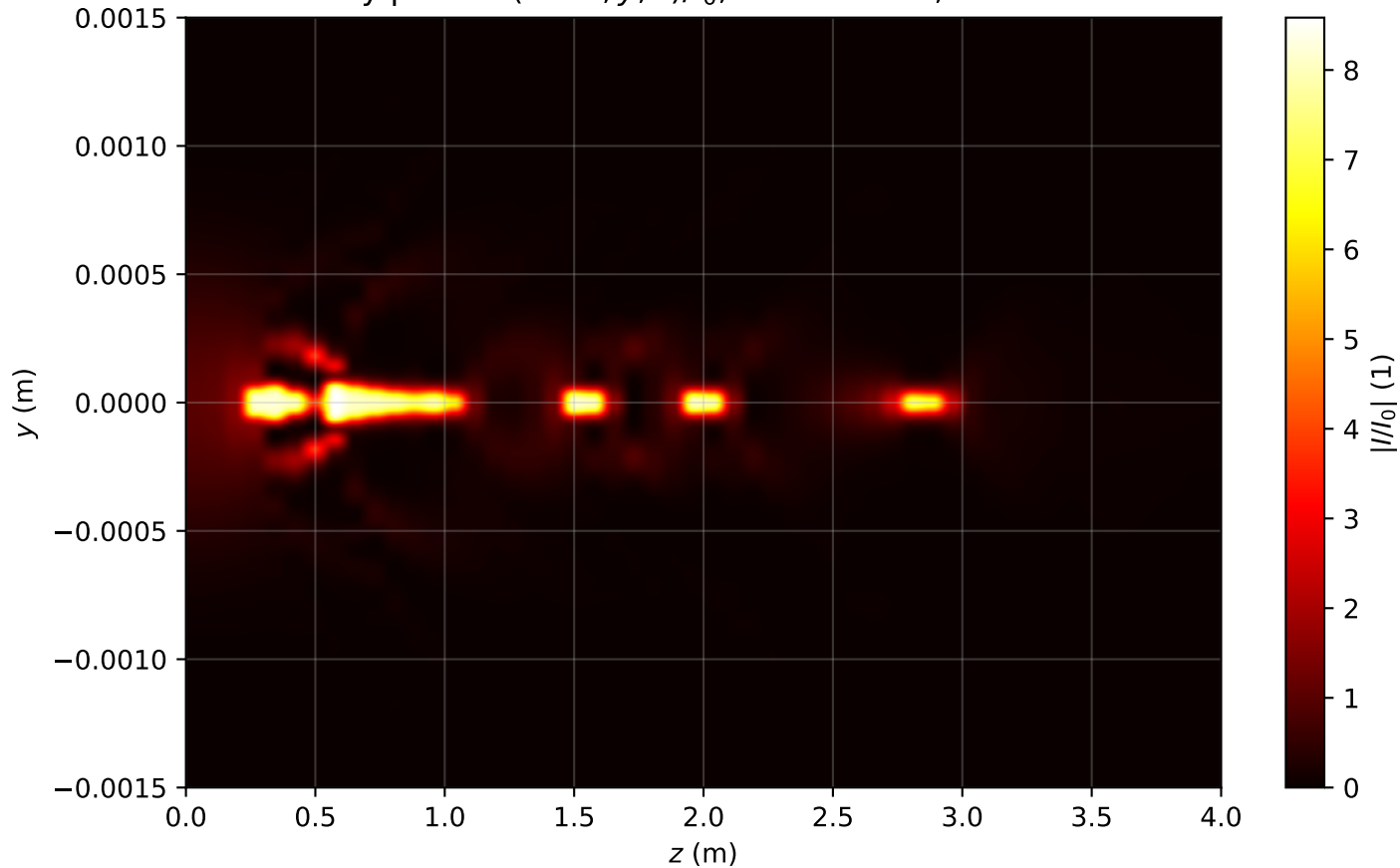
Intensity profile I(x=0, y, z)/I_0 , P_{in}=13.5\text{Pcr} , artificial time
