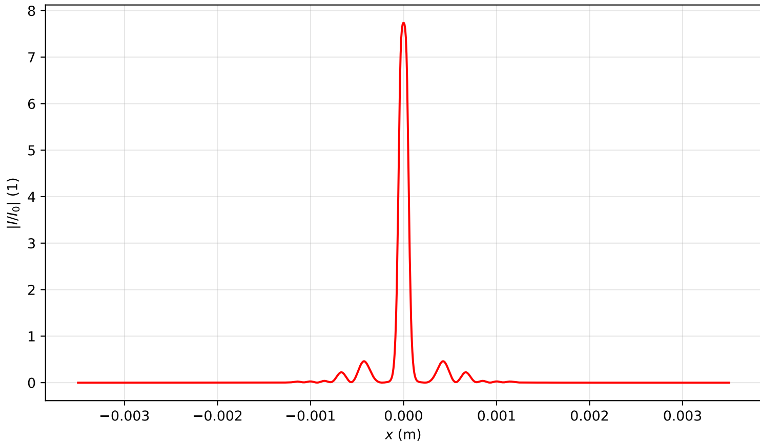
Intensity profile I(x, y = 0, z = 0.716)/I_0 , P_{in}=14.0P_{cr} , artificial time
