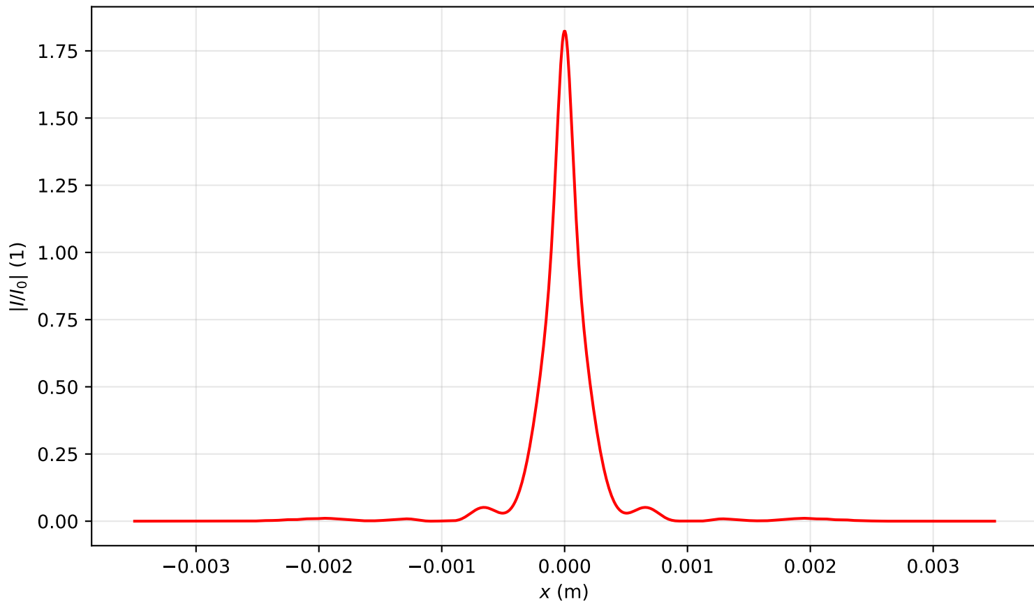
Intensity profile I(x, y = 0, z = 1.433)/I_0 , P_{in}=14.0\text{Pcr} , artificial time
