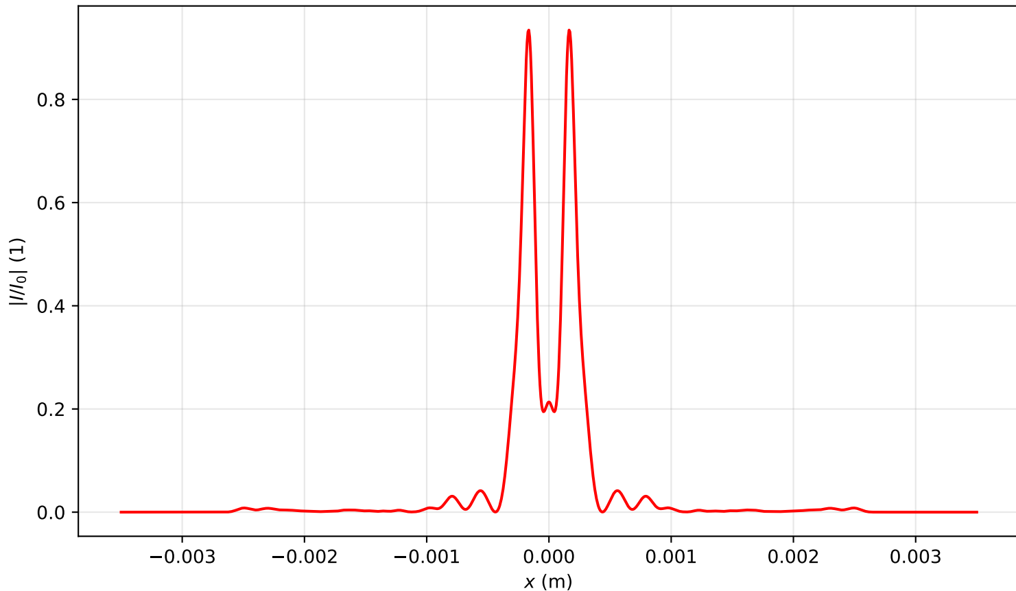
Intensity profile I(x, y = 0, z = 1.672)/I_0 , P_{in}=14.0P_{cr} , artificial time
