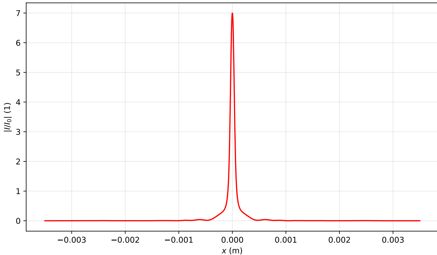
Intensity profile I(x, y = 0, z = 1.911)/I_0 , P_{in}=14.0P_{cr} , artificial time
