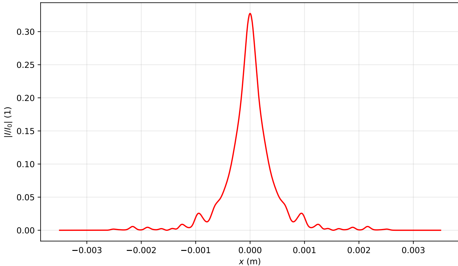
Intensity profile I(x, y = 0, z = 2.388)/I_0 , P_{in}=14.0\text{Pcr} , artificial time
