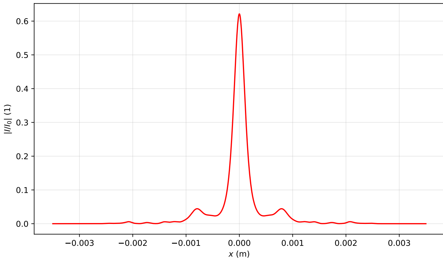
Intensity profile I(x, y = 0, z = 2.627)/I_0 , P_{in}=14.0P_{cr} , artificial time
