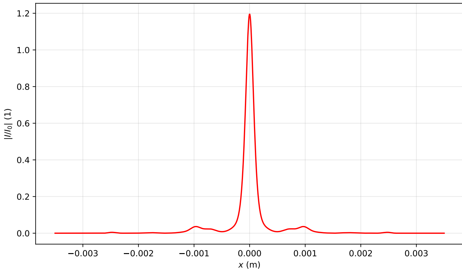
Intensity profile I(x, y = 0, z = 2.866)/I_0 , P_{in}=14.0P_{cr} , artificial time
