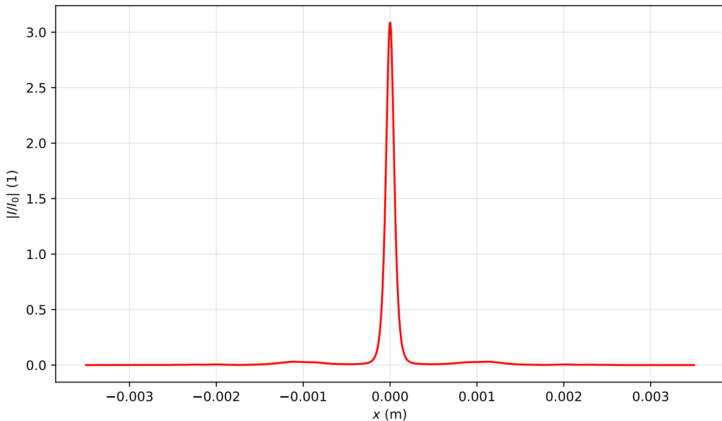
Intensity profile I(x, y = 0, z = 3.105)/I_0 , P_{in}=14.0P_{cr} , artificial time
