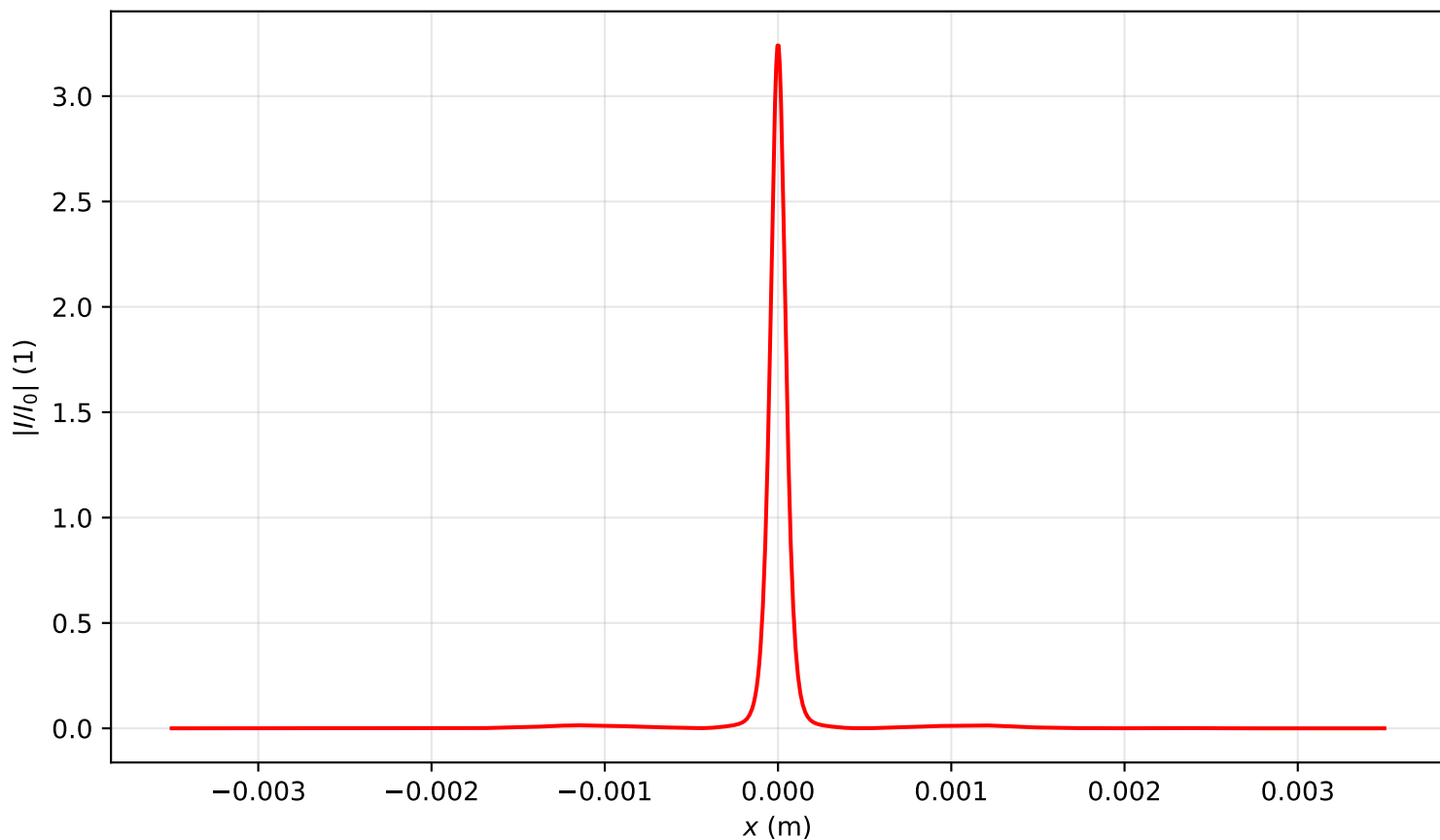
Intensity profile I(x, y = 0, z = 3.344)/I_0 , P_{in}=14.0P_{cr} , artificial time
