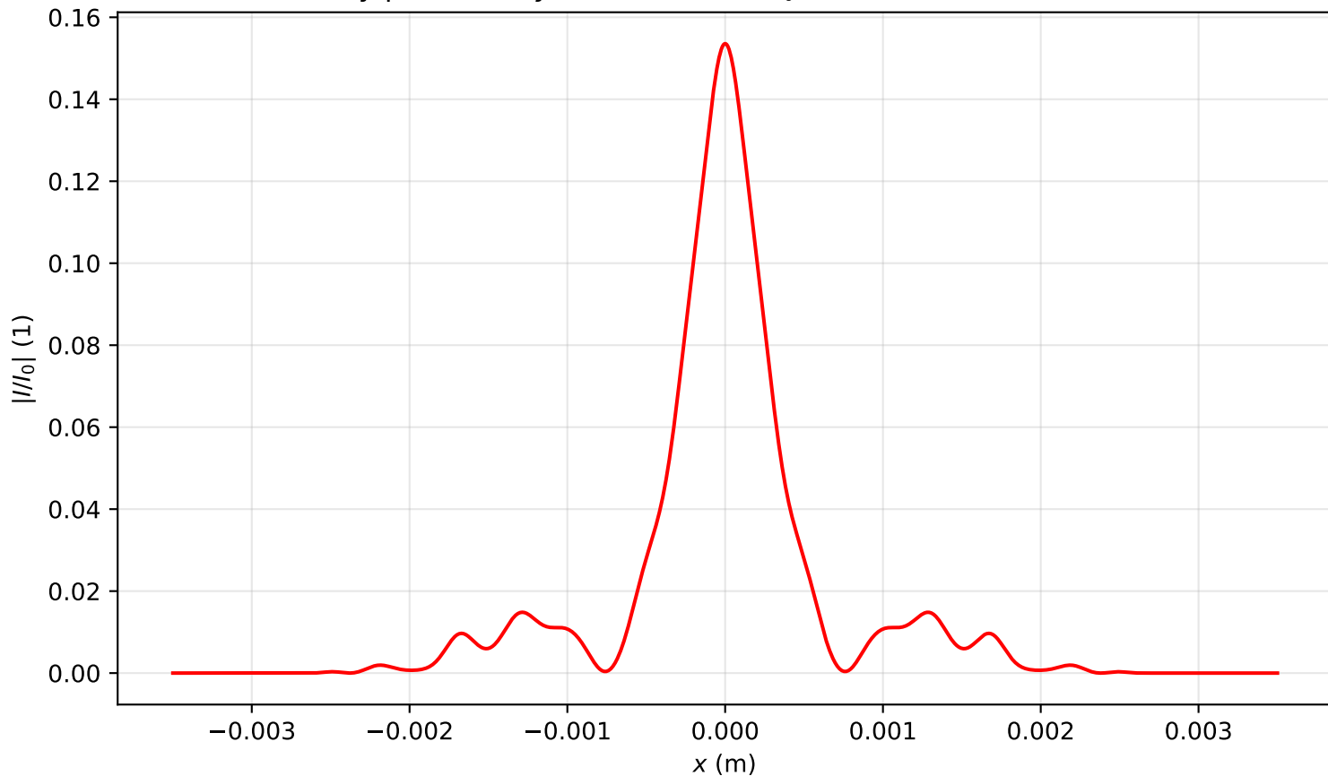
Intensity profile I(x, y = 0, z = 3.821)/I_0 , P_{in}=14.0P_{cr} , artificial time
