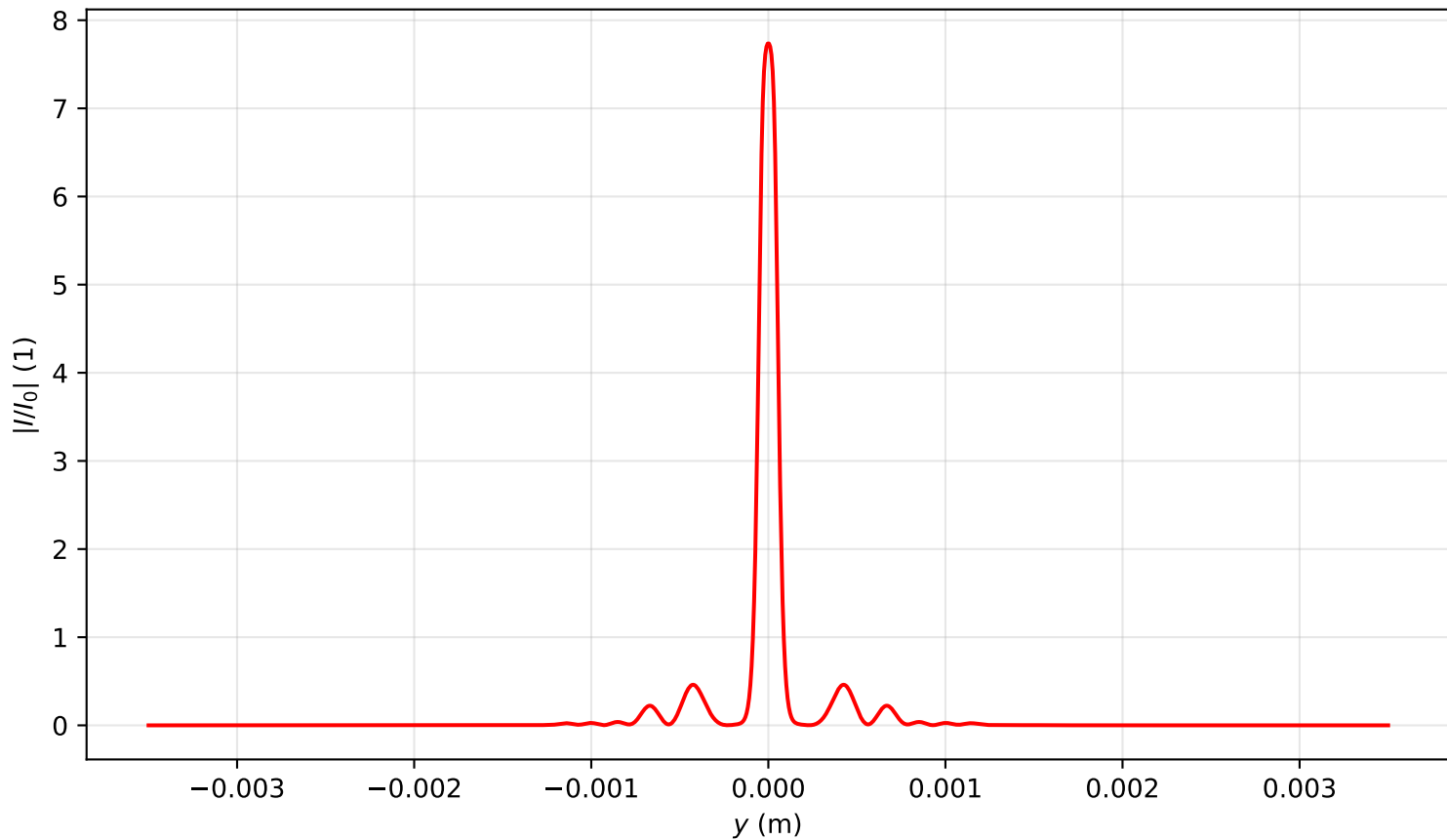
Intensity profile I(x=0, y, z=0.716)/I_0 , P_{in}=14.0P_{cr} , artificial time
