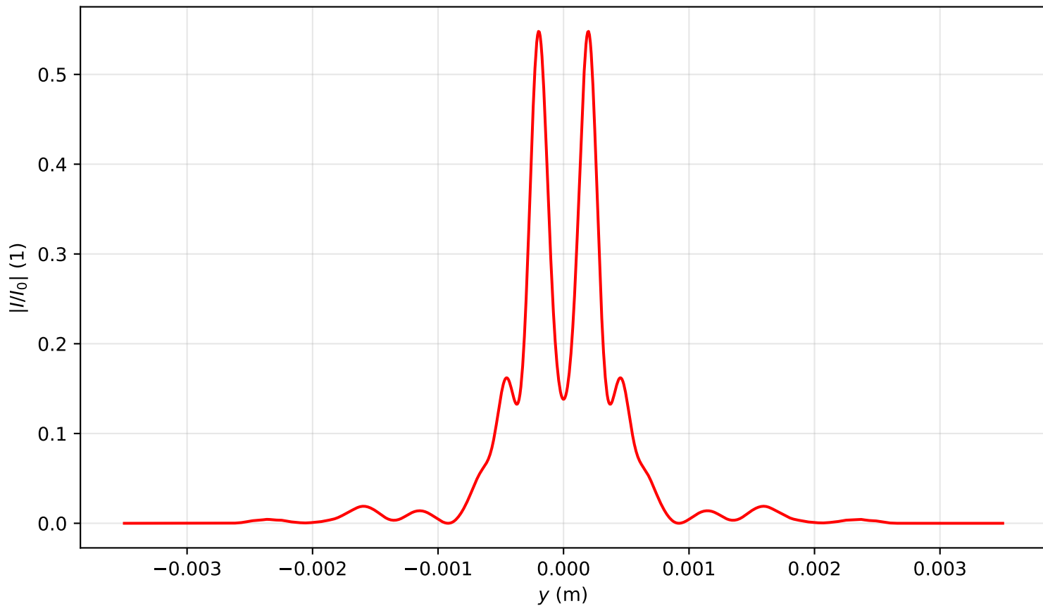
Intensity profile I(x=0, y, z=1.194)/I_0 , P_{in}=14.0P_{cr} , artificial time
