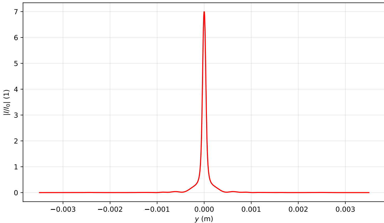
Intensity profile I(x=0, y, z=1.911)/I_0 , P_{in}=14.0P_{cr} , artificial time
