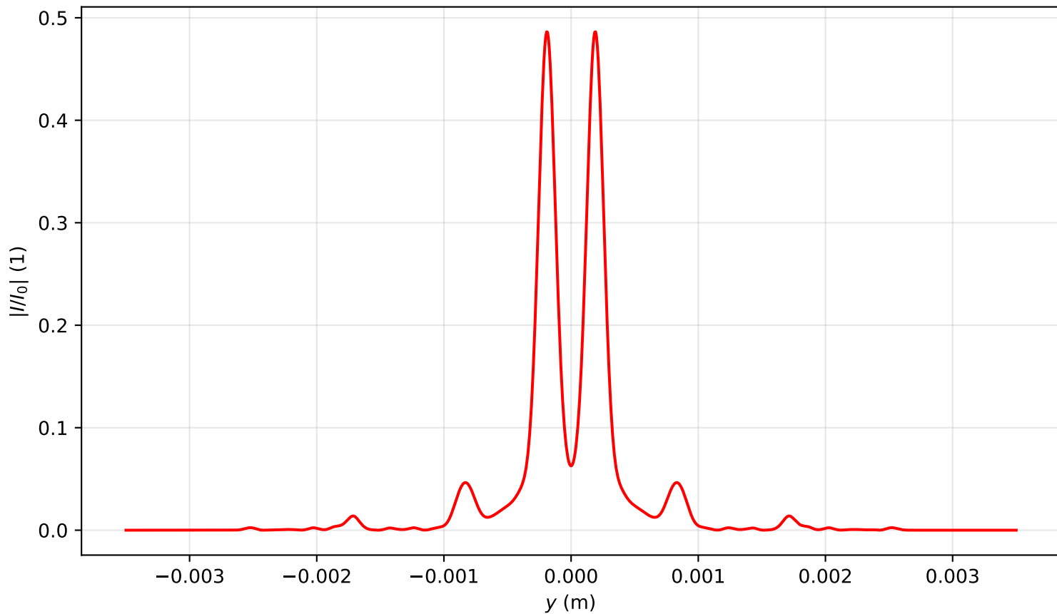
Intensity profile I(x=0, y, z=2.149)/I_0 , P_{in}=14.0P_{cr} , artificial time
