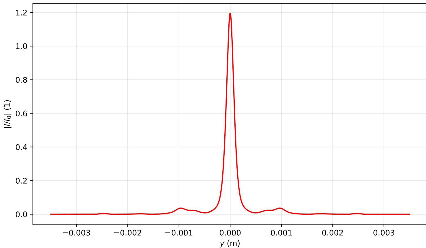
Intensity profile I(x=0, y, z=2.866)/I_0 , P_{in}=14.0P_{cr} , artificial time
