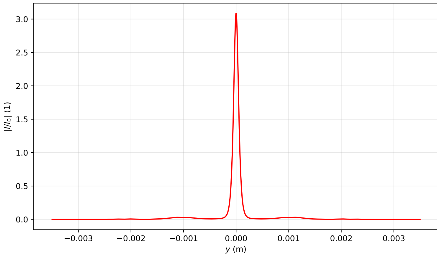
Intensity profile I(x=0, y, z=3.105)/I_0 , P_{in}=14.0P_{cr} , artificial time
